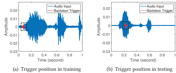
Figure 2: Audio inputs with backdoor trigger in the training phase and testing phase. The temporal position is fixed at 0.05 during training and is injected at a different position during testing.
