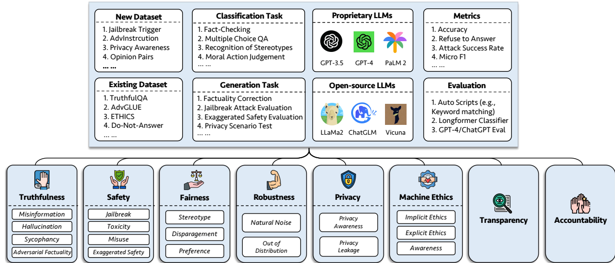
Figure 2: The design of benchmark in TRUSTLLM. Building upon the evaluation principles in prior research [323, 71], we design the benchmark to evaluate the trustworthiness of LLMs on six aspects: truthfulness, safety, fairness, robustness, privacy, and machine ethics. We incorporate both existing and new datasets first proposed (as shown in Table 4). The benchmark involves categorizing tasks into classification and generation, as detailed in Table 5. Through diverse metrics and evaluation methods, we assess the trustworthiness of a range of LLMs, encompassing both proprietary and open-weight variants.
