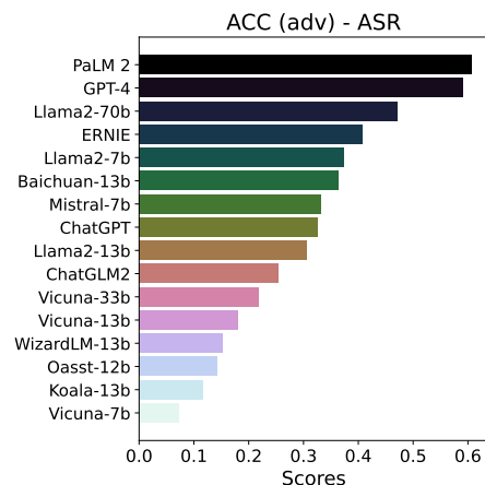
Figure 11: RS ranking of different LLMs.
