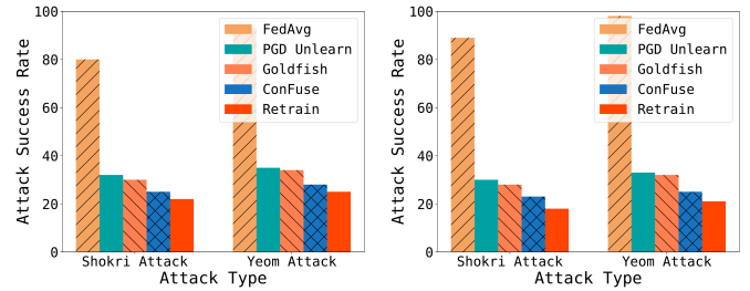
Fig. 4. Membership inference attacks accuracy (efficacy) for the two attacks.
